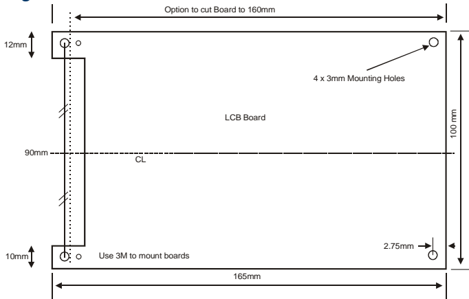
Figure 2.5 LCB Board
