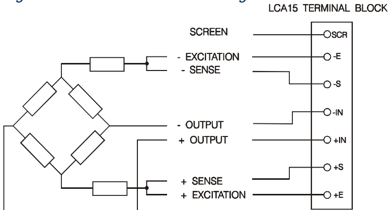
Figure 2.7 The 6 Wire Strain Gauge
