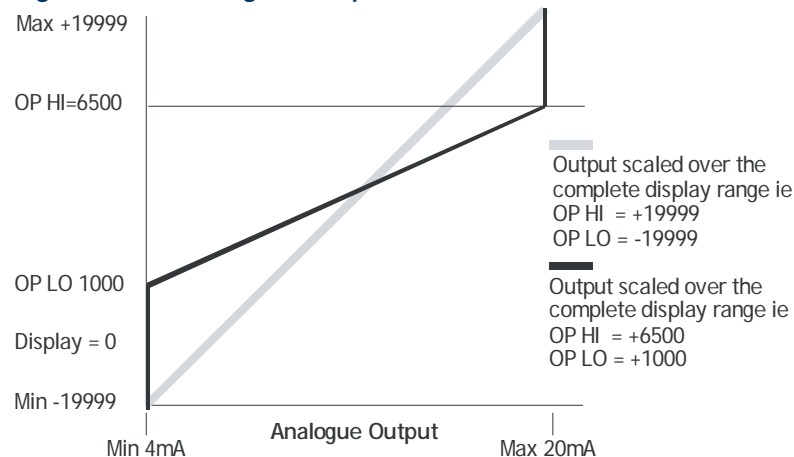
Figure 5.1 Analogue Output
