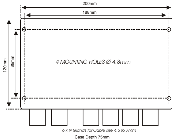
Figure 2.2 IP65-ABS Case (LAB) Dimensions & Mounting Points
