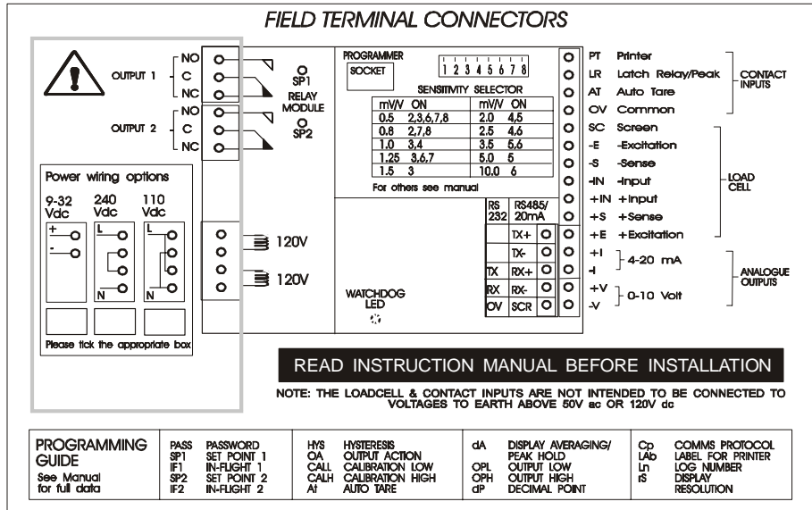
Figure 2.1 The LCA15 Field Connection Terminals
