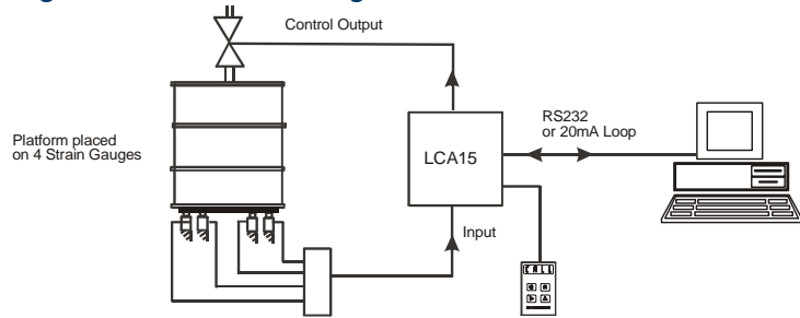
Figure 1.2 Drum Filling
