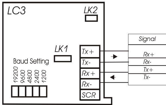
Figure 7.3 The LC3 Isolated RS232/485 - RS485 Mode Connections
