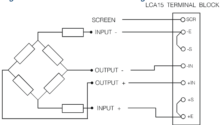
Figure 2.7 The 6 Wire Strain Gauge
