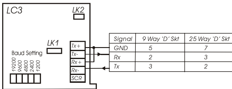
Figure 7.5 RS232 Mode Connection to PC
