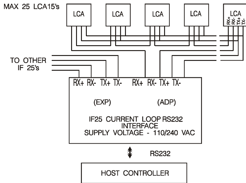
Figure 7.2 Connecting Multiple LCA15s
