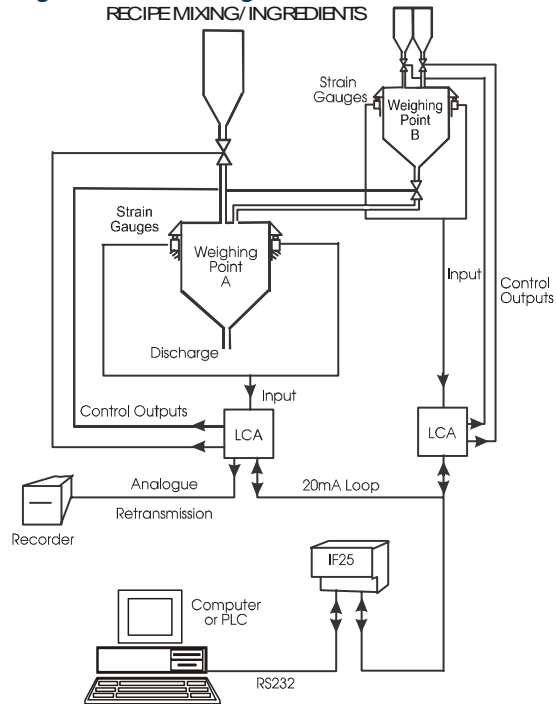
Figure 1.3 Mixing Control
